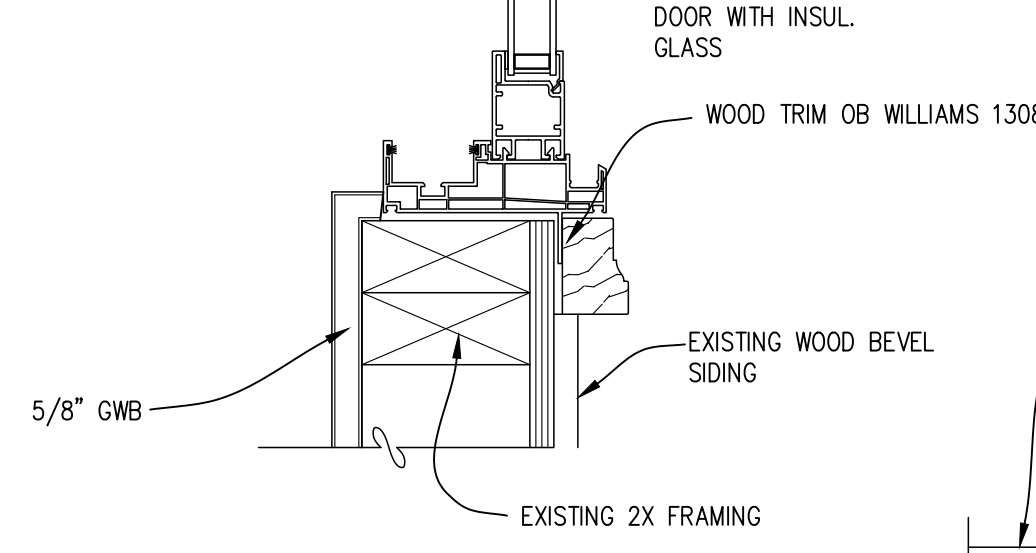
7 JAMB 3" = 1'-0"
