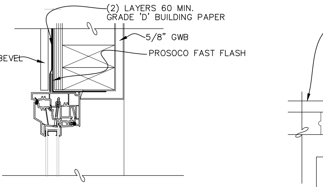
11 JAMB 3" = 1'-0"
